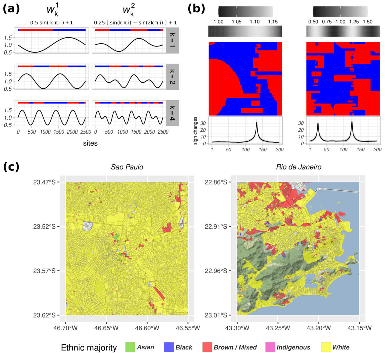
Fig. 1: (a) Stationary states on a one-dimensional lattice with N = 2500 nodes, happiness threshold U_0 = 0 and two families of oscillating weight functions (black curves). Top: final configuration, where agents in state 1 are blue and in state 1, red. (b) Stationary states on a squared lattice of side 200. The weight functions are at the top in greyscale; at the bottom, the mean number of sign changes within each column taken over 50 realizations with different initial distributions of agents states. (c) Topography maps and distribution of majority ethnicity according to 2010 Census for urban areas of Sao Paulo and Rio de Janeiro.
